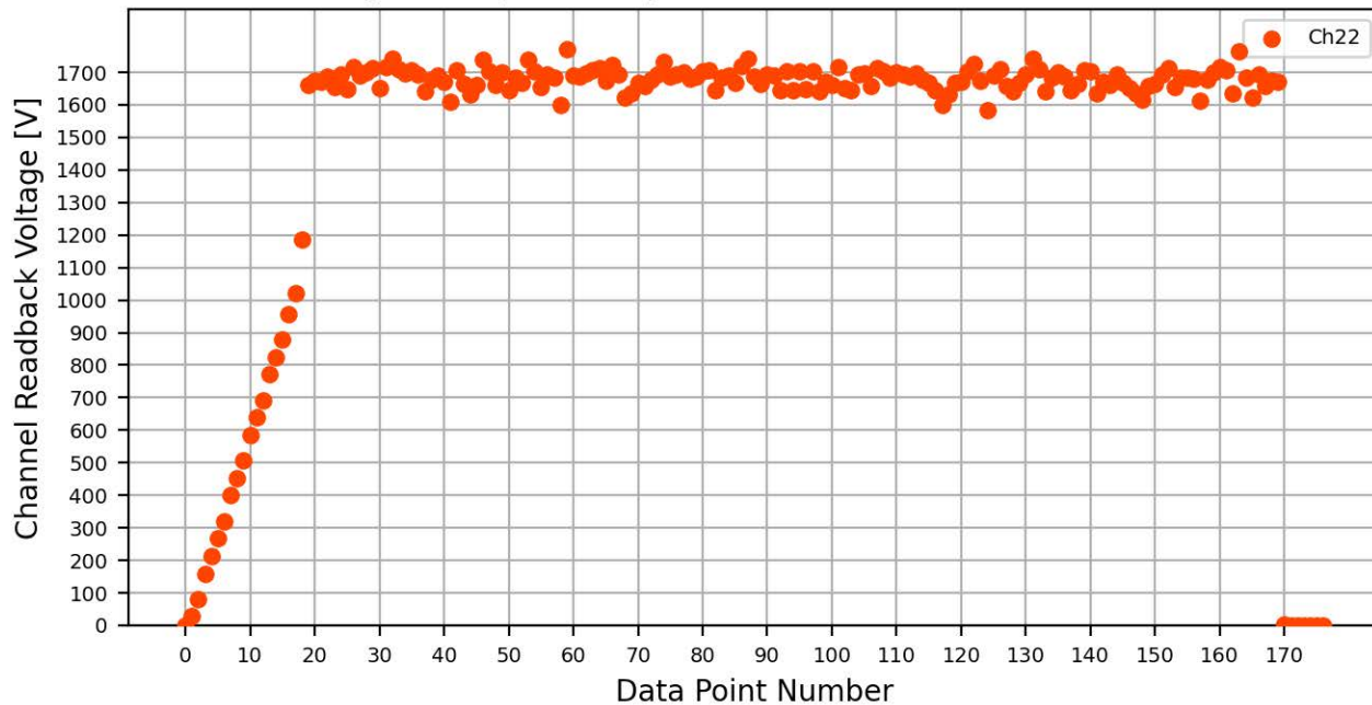
Voltage Ramp Test (Python) Bd #766, Slot #1, Ch #22
