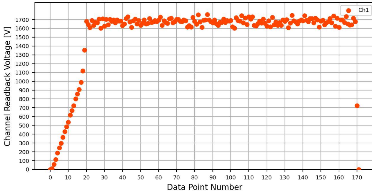
Voltage Ramp Test (Python) Bd #766, Slot #1, Ch #1
