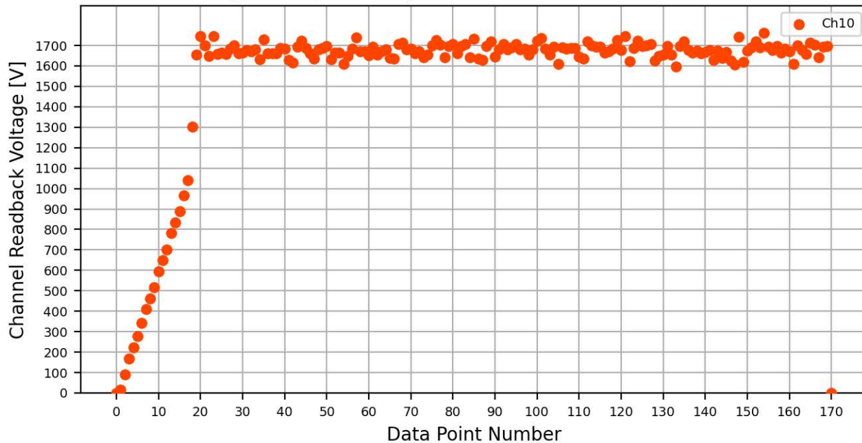
Voltage Ramp Test (Python) Bd #766, Slot #1, Ch #10
