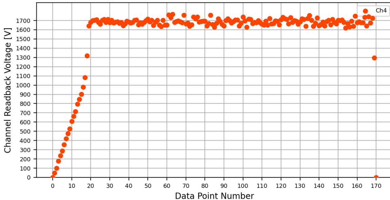
Voltage Ramp Test (Python) Bd #766, Slot #1, Ch #4
