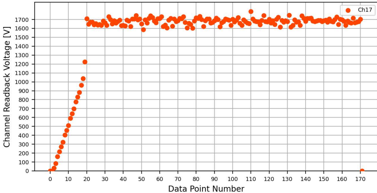
Voltage Ramp Test (Python) Bd #766, Slot #1, Ch #17
