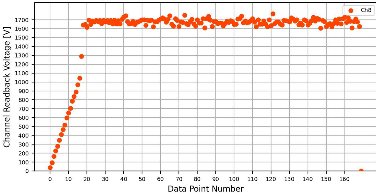
Voltage Ramp Test (Python) Bd #766, Slot #1, Ch #8
