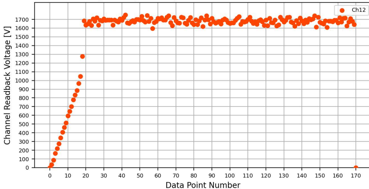
Voltage Ramp Test (Python) Bd #766, Slot #1, Ch #12
