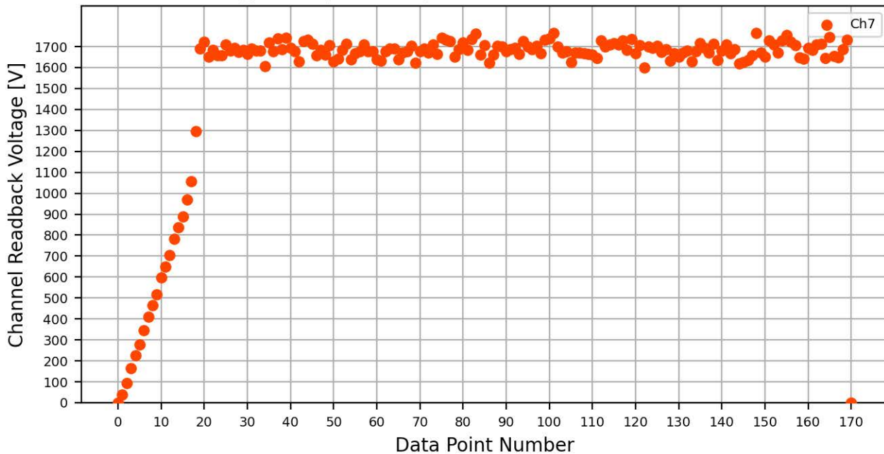
Voltage Ramp Test (Python) Bd #766, Slot #1, Ch #7
