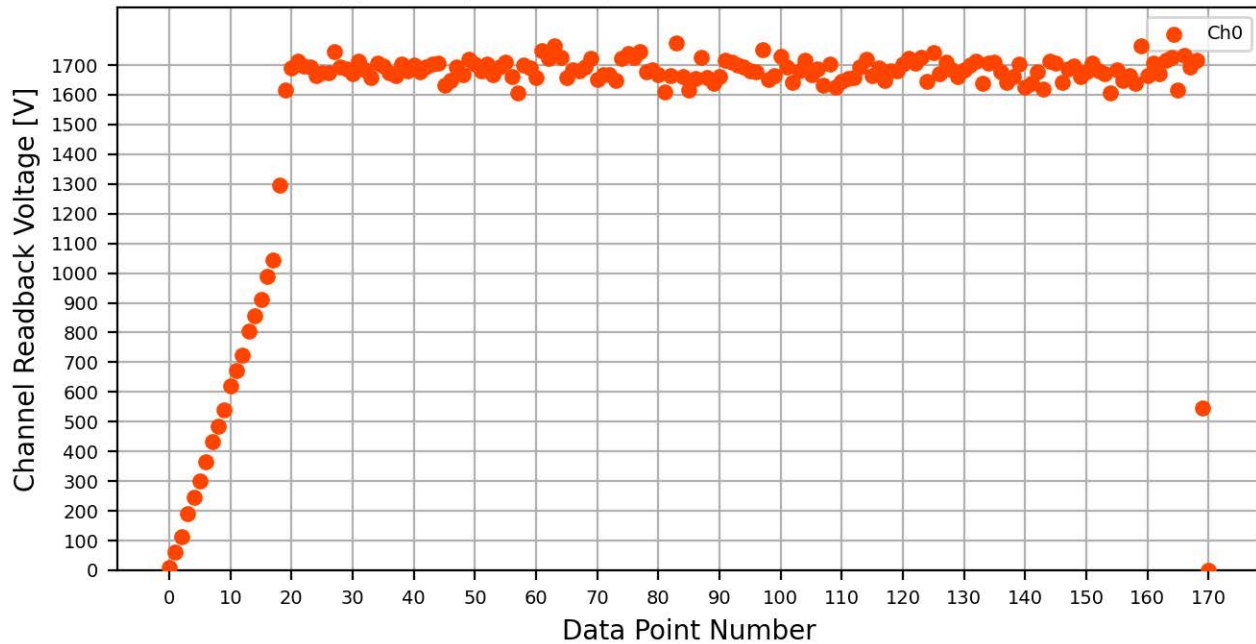
Voltage Ramp Test (Python) Bd #766, Slot #1, Ch #0
