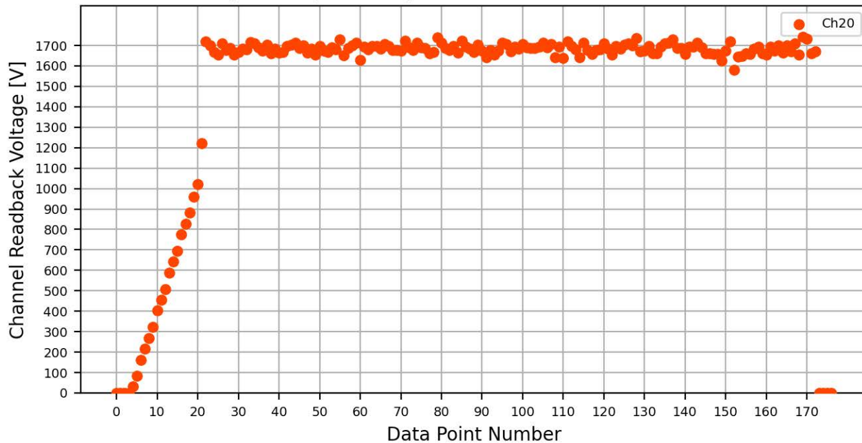
Voltage Ramp Test (Python) Bd #766, Slot #1, Ch #20
