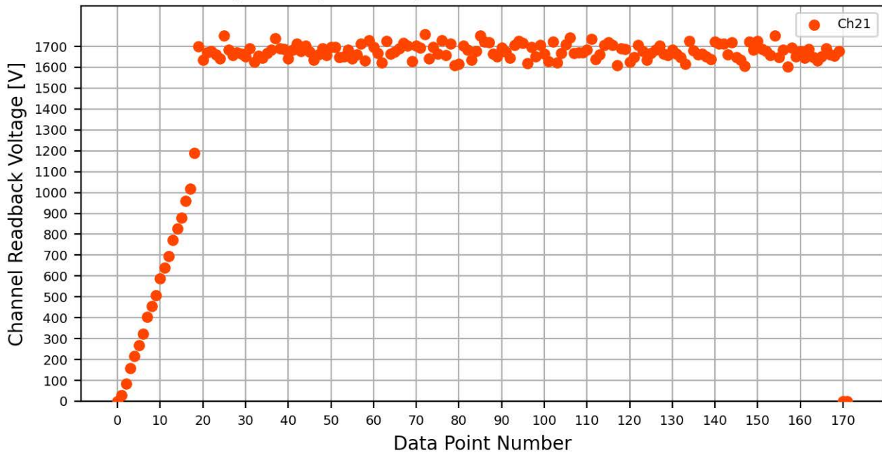
Voltage Ramp Test (Python) Bd #766, Slot #1, Ch #21
