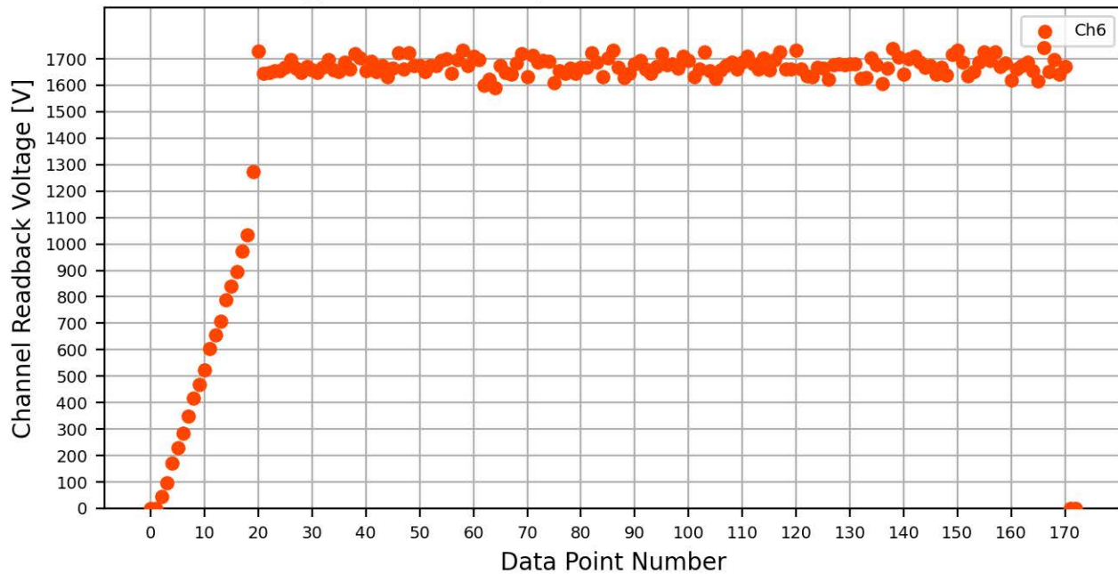
Voltage Ramp Test (Python) Bd #766, Slot #1, Ch #6
