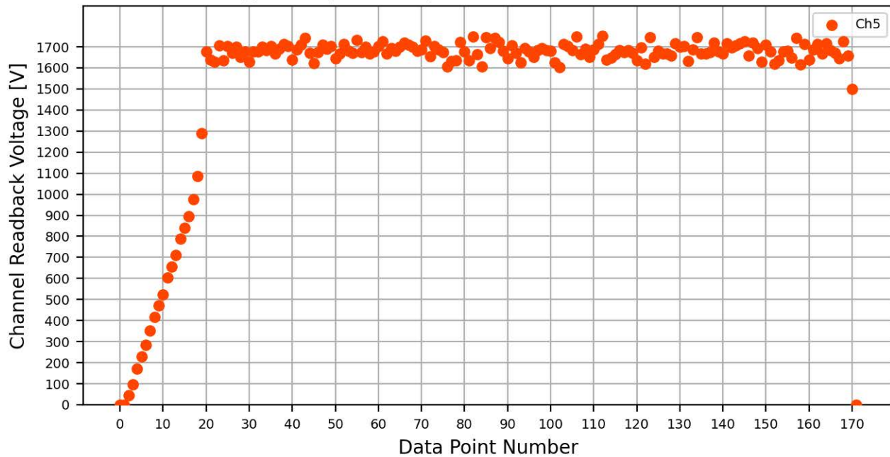
Voltage Ramp Test (Python) Bd #766, Slot #1, Ch #5
