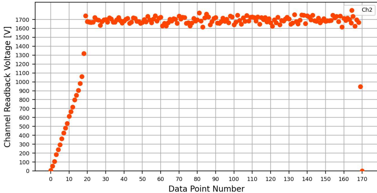
Voltage Ramp Test (Python) Bd #766, Slot #1, Ch #2
