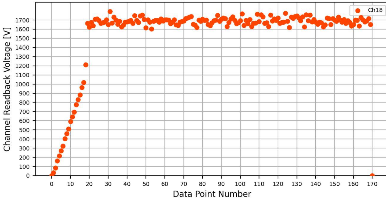
Voltage Ramp Test (Python) Bd #766, Slot #1, Ch #18
