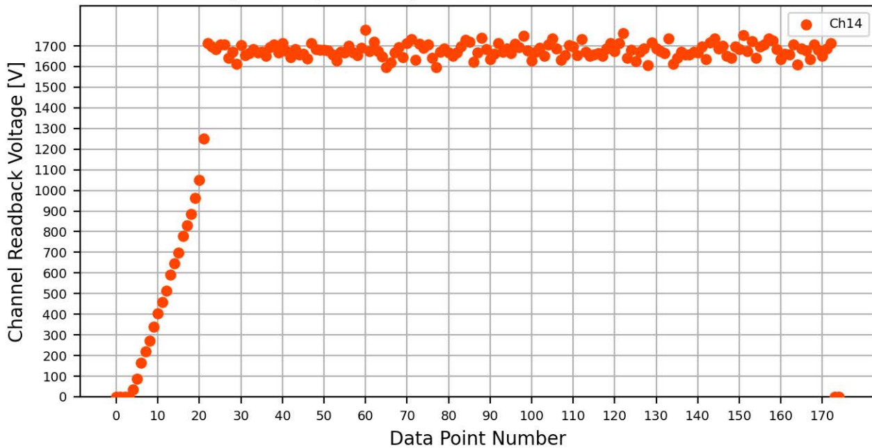
Voltage Ramp Test (Python) Bd #766, Slot #1, Ch #14
