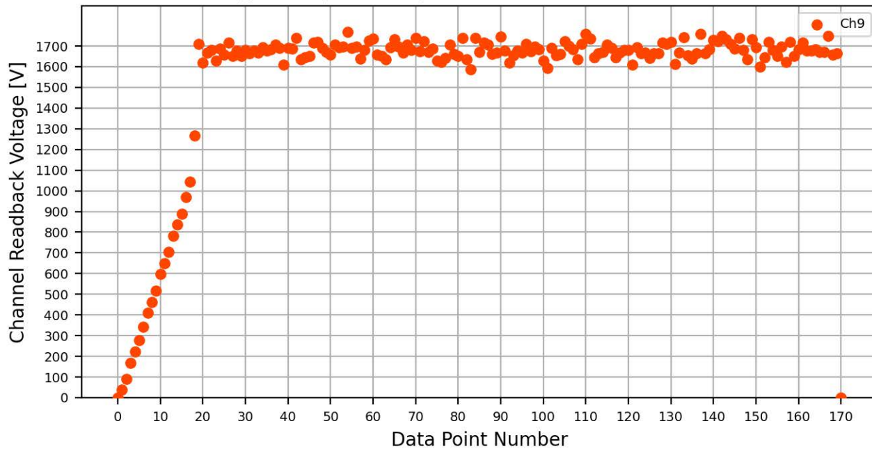
Voltage Ramp Test (Python) Bd #766, Slot #1, Ch #9
