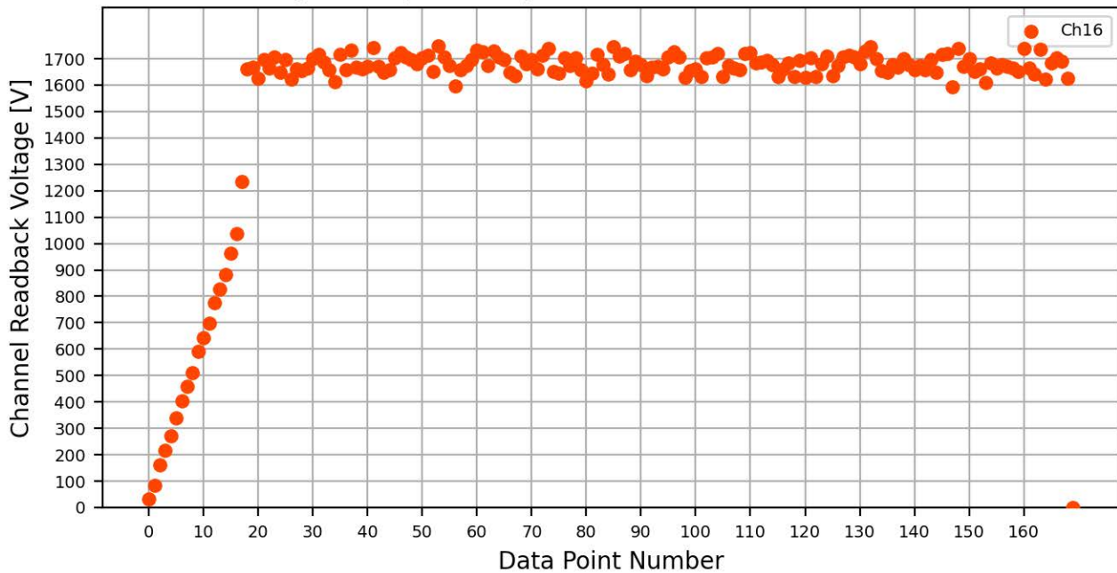
Voltage Ramp Test (Python) Bd #766, Slot #1, Ch #16
