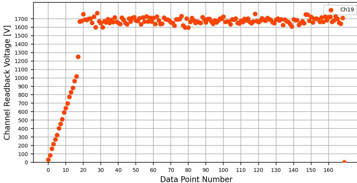
Voltage Ramp Test (Python) Bd #766, Slot #1, Ch #19
