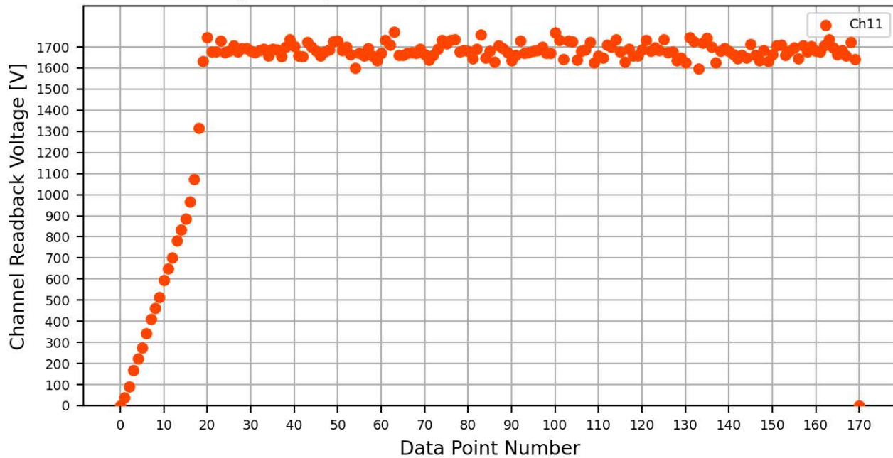
Voltage Ramp Test (Python) Bd #766, Slot #1, Ch #11
